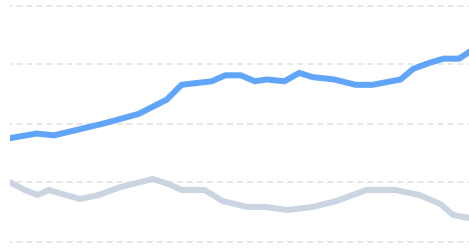
Line Chart >
